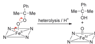
Scheme 2. Heterolytic O–O bond cleavage of nonheme iron(II) (hydro/alkyl)peroxo complexes.
